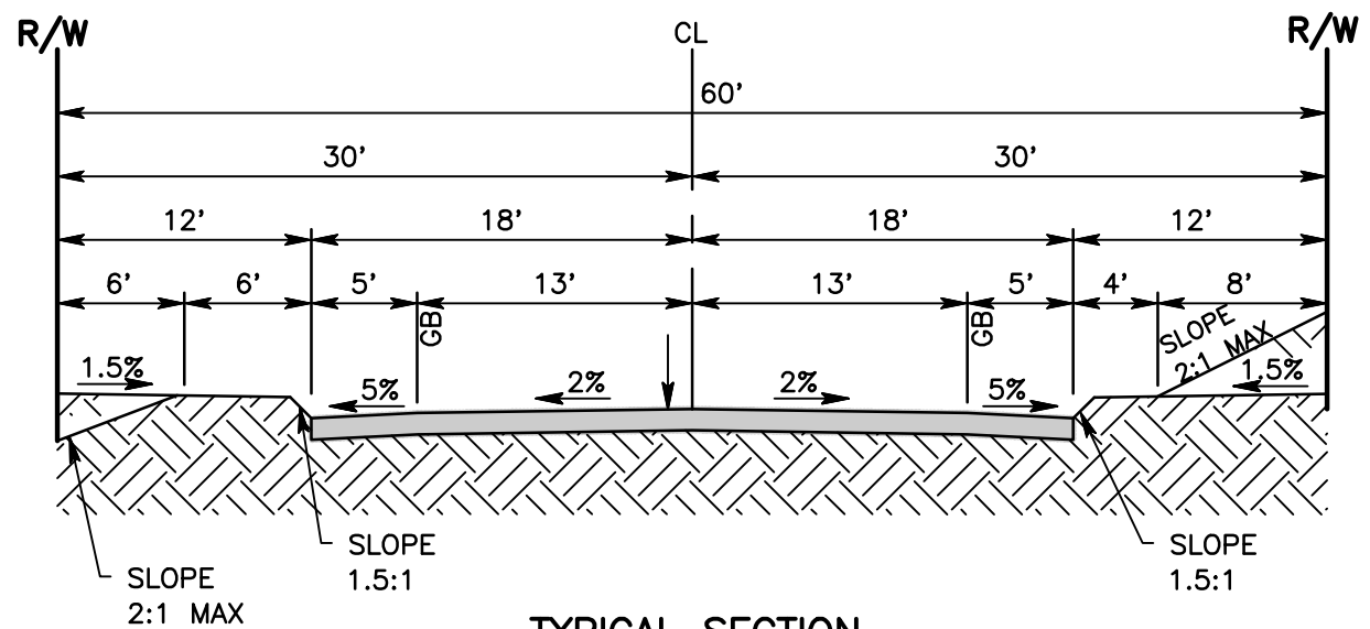
TYPICAL SECTION
