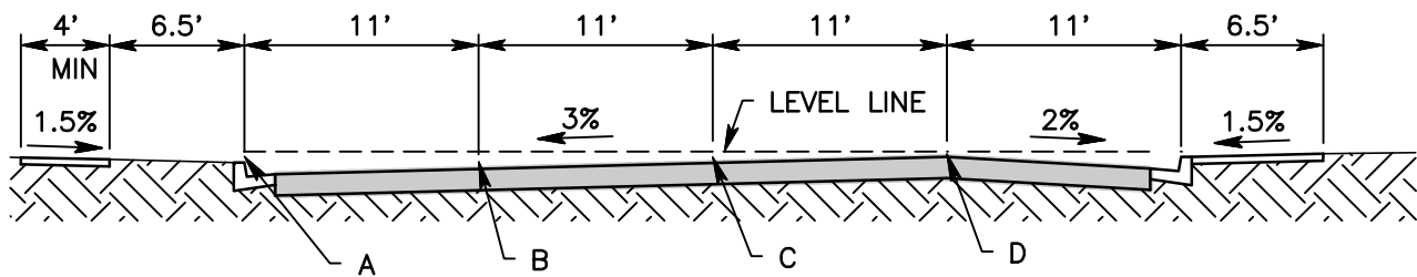
TYPICAL SECTION TILT
